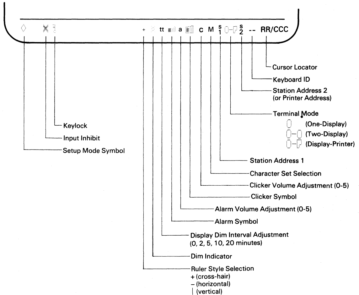
Figure 1-4. Symbols in Setup Mode
